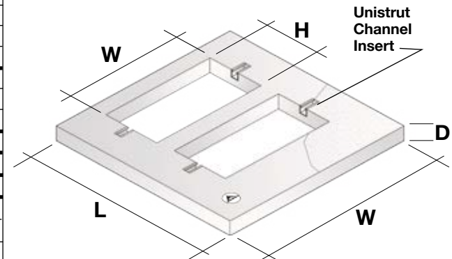
TYPE II Dual Window-Top & Bottom
